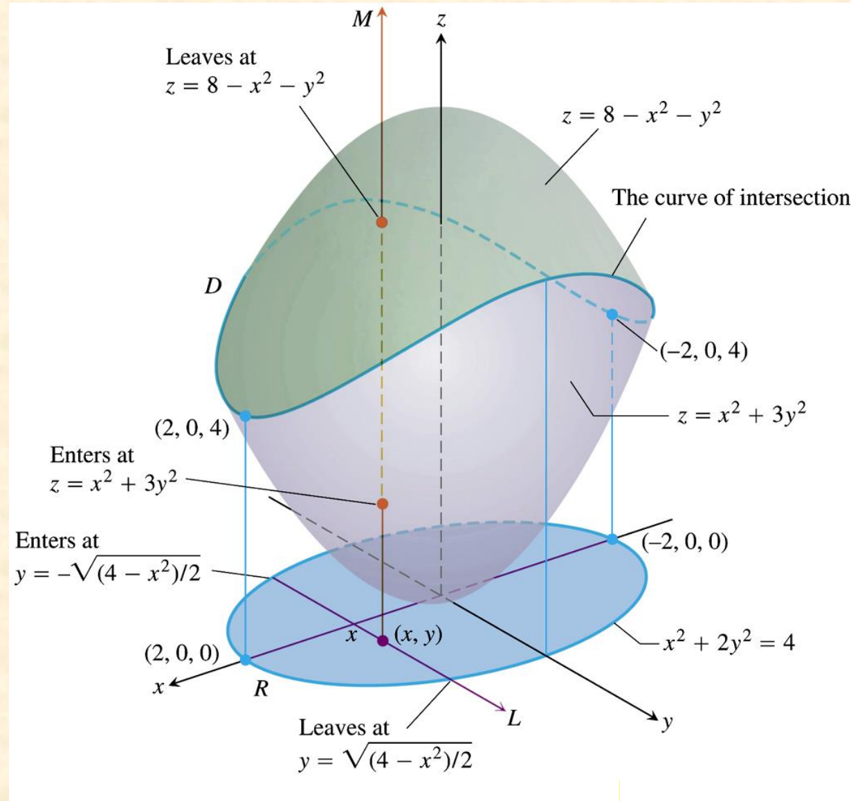
FIGURE 15.28 The volume of the region enclosed by two paraboloids, calculated in Example 1.
