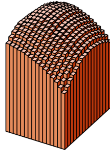
(c) n = 256
