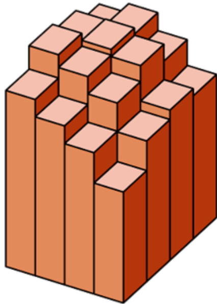
(a) n = 16
