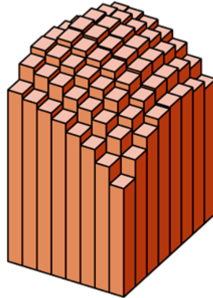
(b) n = 64
